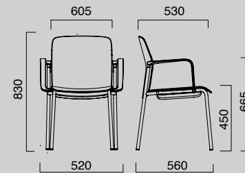
KM4LPA 4 Legs with Arms
