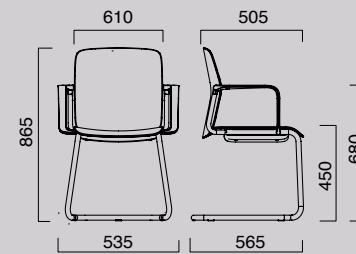
KMCPA Cantilever Base with Arms
