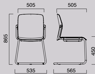
KMCP Cantilever Base
